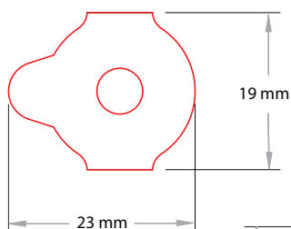
Shape: 1698 Round 19 mm x 23 mm
