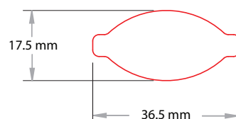
Shape: 1777 Football 17.5 mm x 36.5 mm
